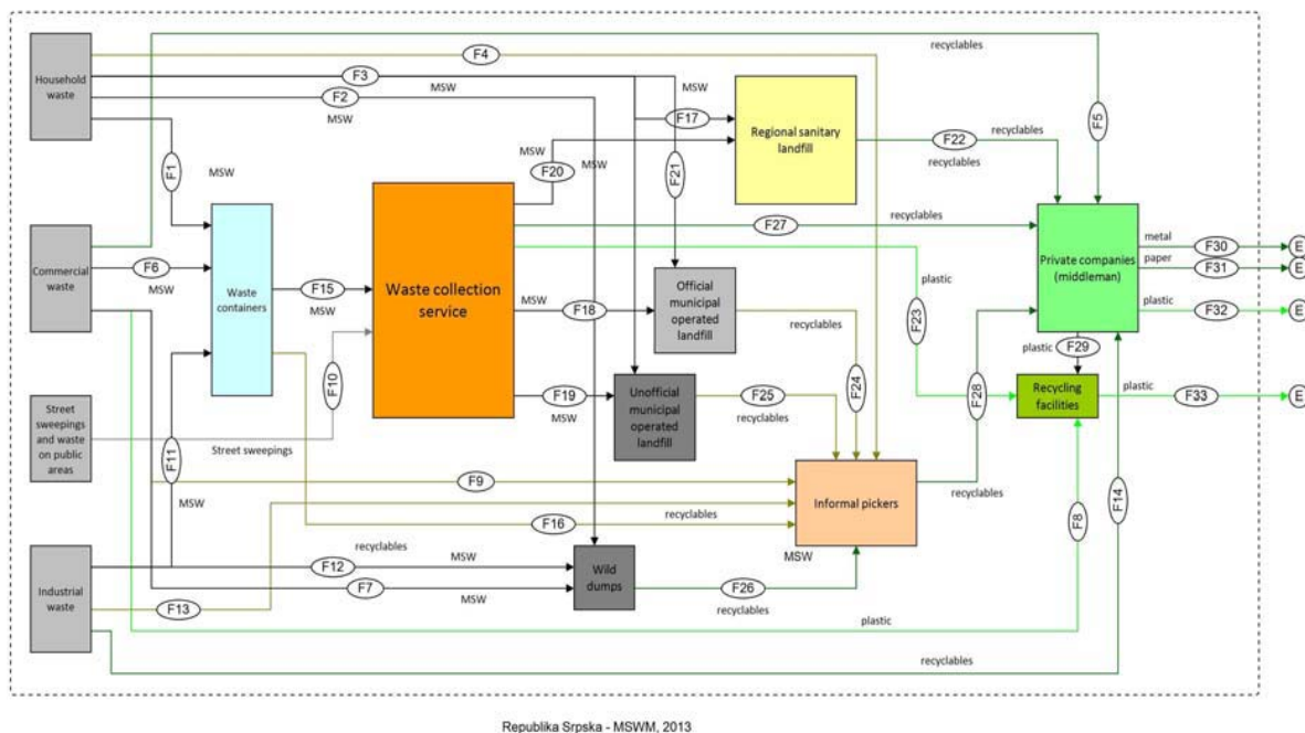
Figure 2. Material Flow Diagram for MSWM in Republika Srpska (Topić, 2014)
